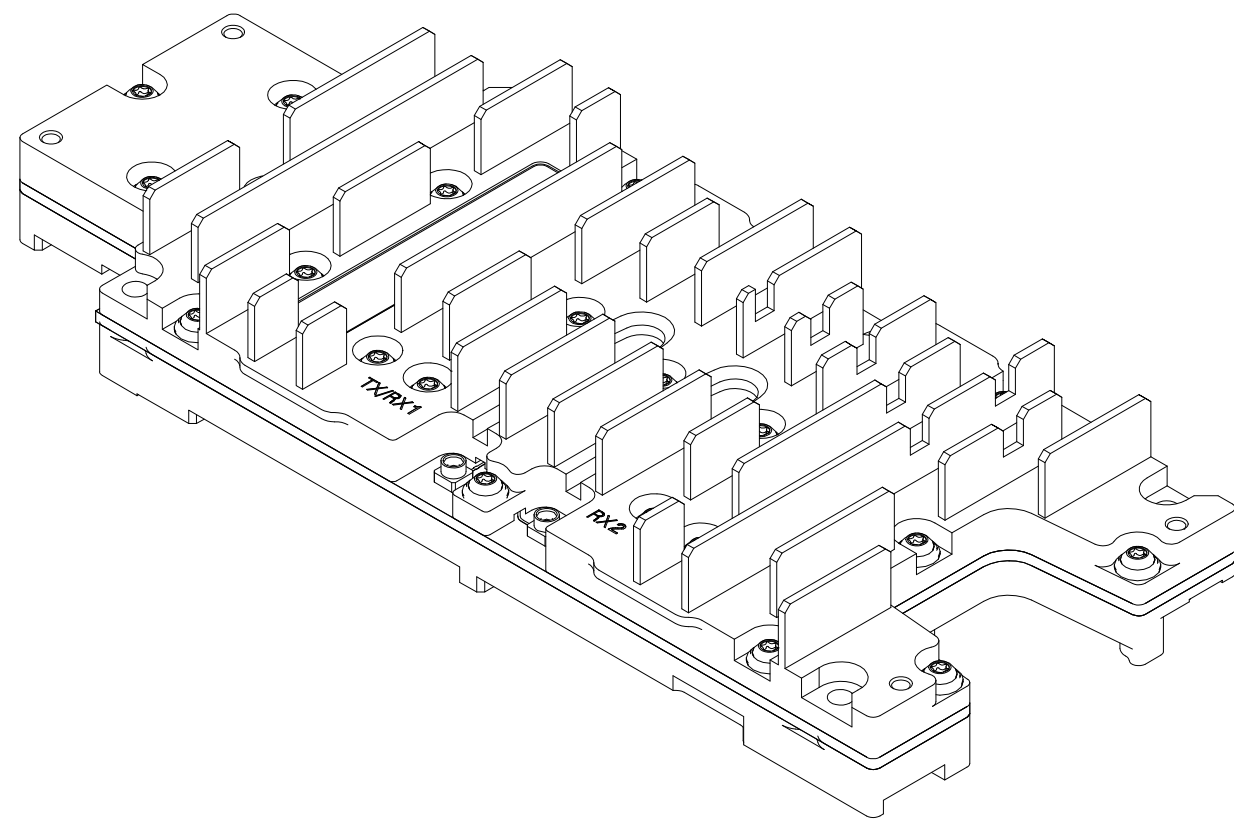
ISOMETRIC VIEW
