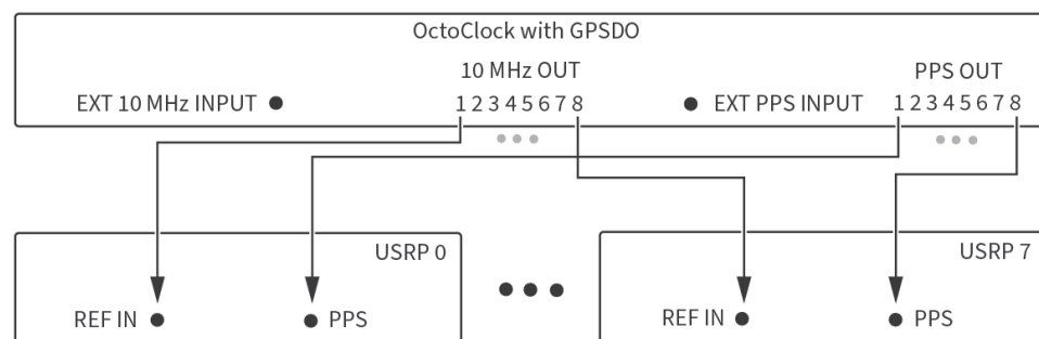
Figure 11. 10 MHz and PPS Connections (16x16)
