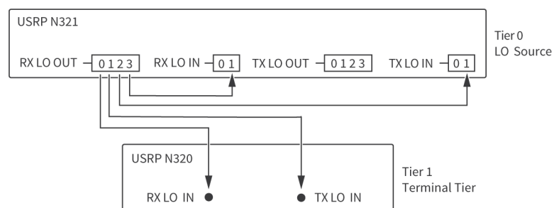
Figure 14. LO Sharing (4x4)
