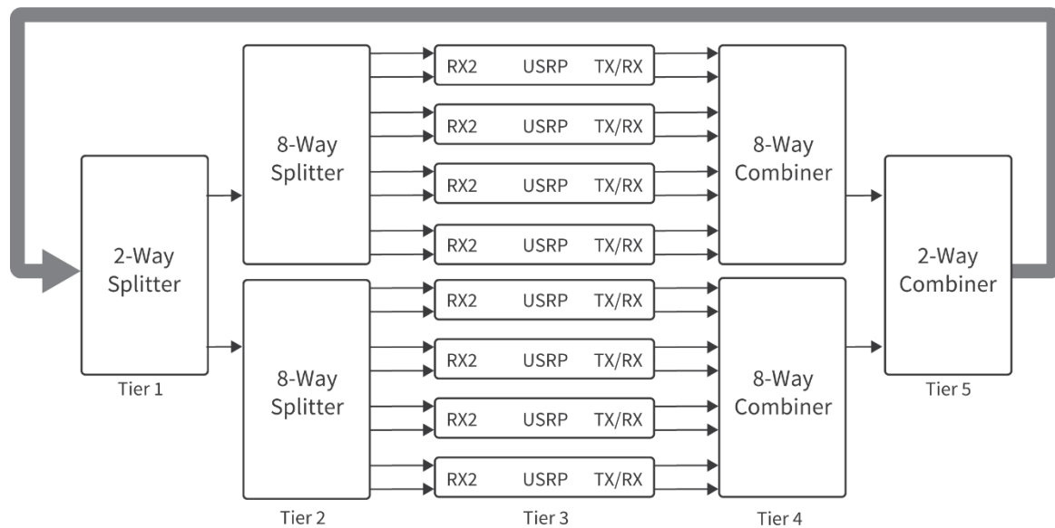
Figure 7. MIMO Loopback (16x16)
