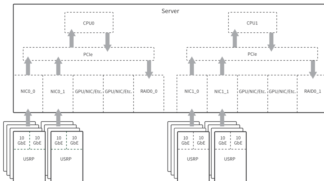
Figure 18. Overview of Dataflow between the USRPs and the Server
