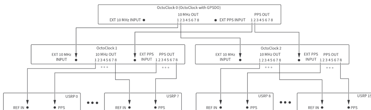
Figure 12. 10 MHz and PPS Connections (32x32)
