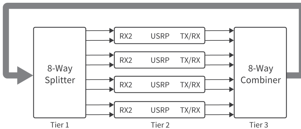
Figure 6. MIMO Loopback (8x8)
