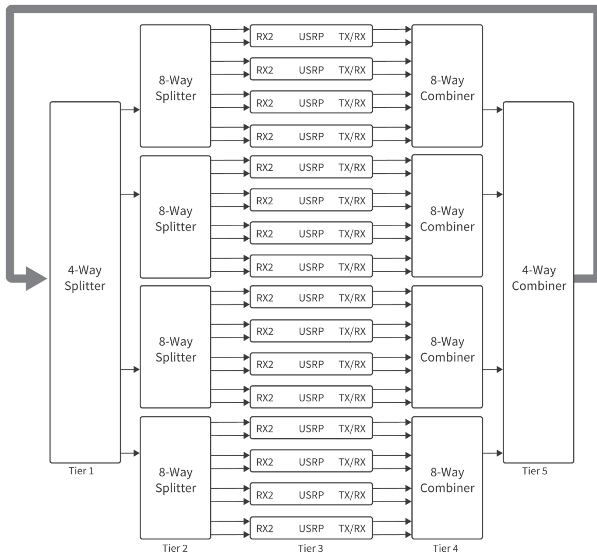
Figure 8. MIMO Loopback (32x32)
