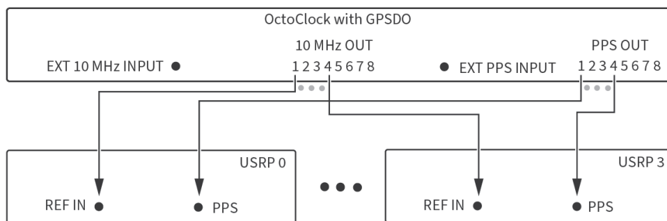
Figure 10. 10 MHz and PPS Connections (8x8)
