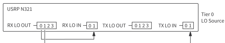
Figure 13. LO Sharing (2x2)
