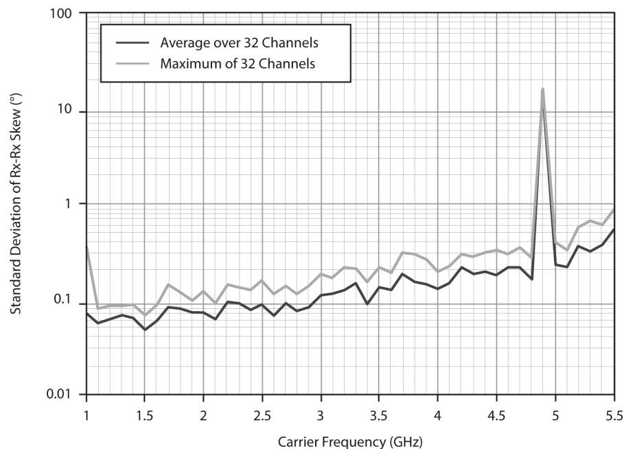
Figure 22. Standard Deviation in Short-Term Rx-Rx Phase Skew as a Function of Carrier Frequency
