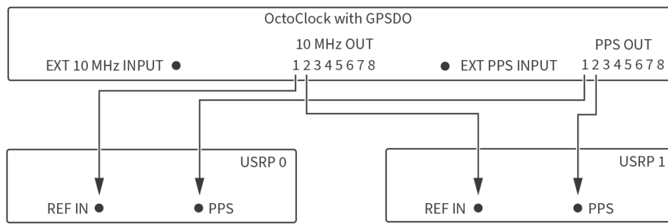
Figure 9. 10 MHz and PPS Connections (4x4)
