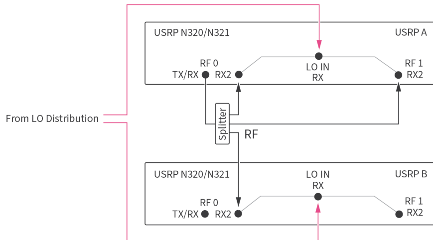
Figure 19. RF Configuration for Stability Measurements
